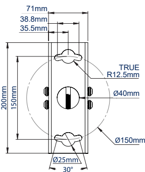
Ceiling / WALL PLATE
