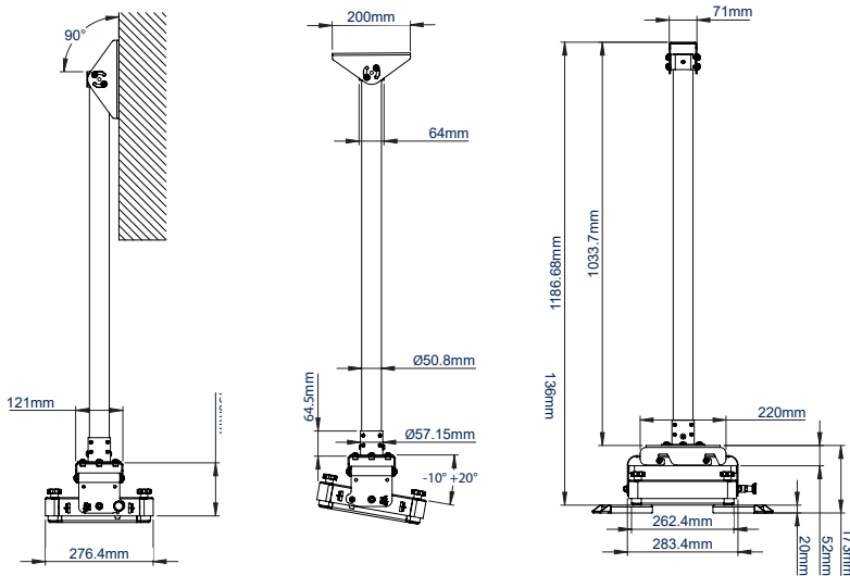
SIDE VIEW WALL MOUNTED
