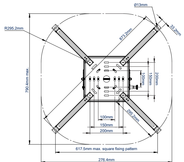
BOTTOM VIEW WITH LARGE EXTENSION LEGS
