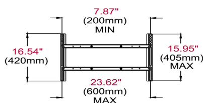
ADAPTOR PLATE
