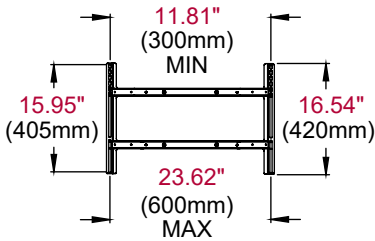
ADAPTOR PLATE
